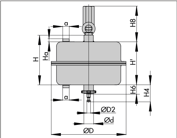
Fig. 4: 1000 cm² actuator area, with adjustable travel stop
