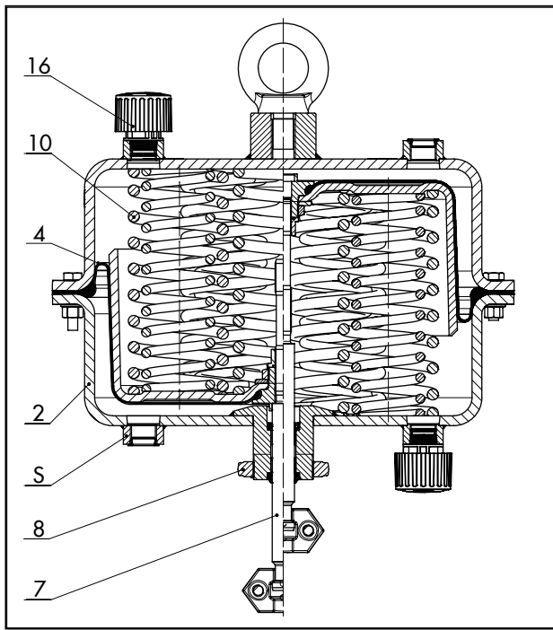
Fig. 2: Type 3271 with 1000 cm 2 actuator area
