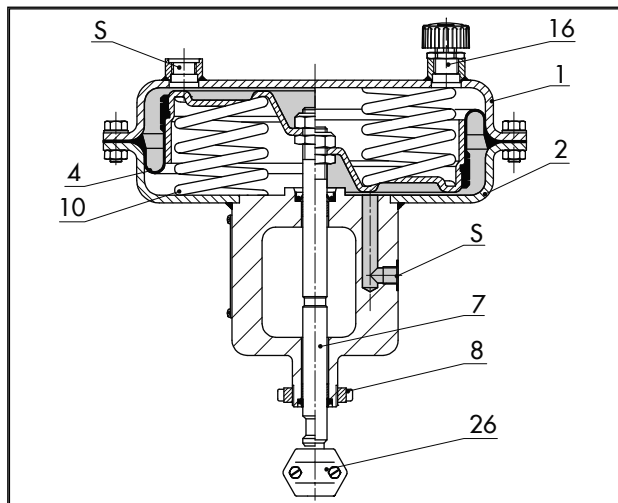
Fig. 9: Type 3277 for direct attachment of accessories (example shows actuator with 350 \text{ cm}^2 )
