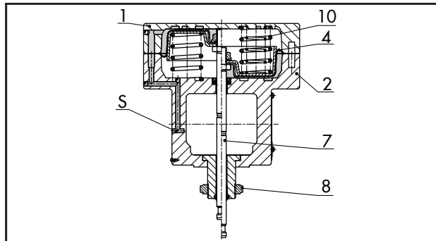
Fig. 8: Type 3277-5 for direct attachment of accessories ( 120 \text{ cm}^2 )
