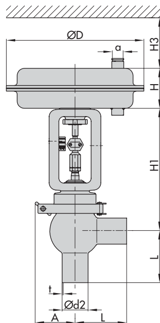
Type 3347-1 Control Valve with welding ends
