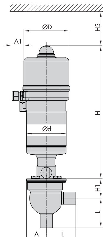
Type 3347/3379/3724 Control Valve with welding ends and bolted bonnet · Bar stock version
