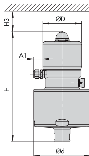
Type 3379 Actuator with Type 3724 Positioner
