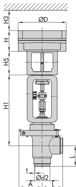
Type 3347-7 Control Valve with welding ends
