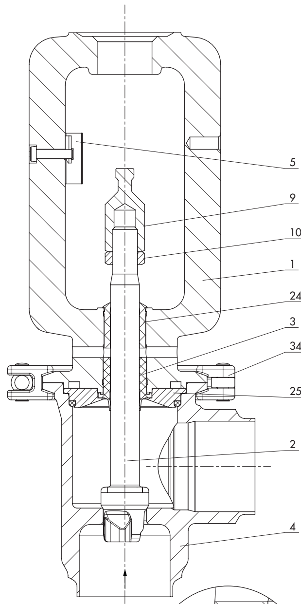
Fig. 5: Type 3347 Valve, cast body, PEEK-guided version
