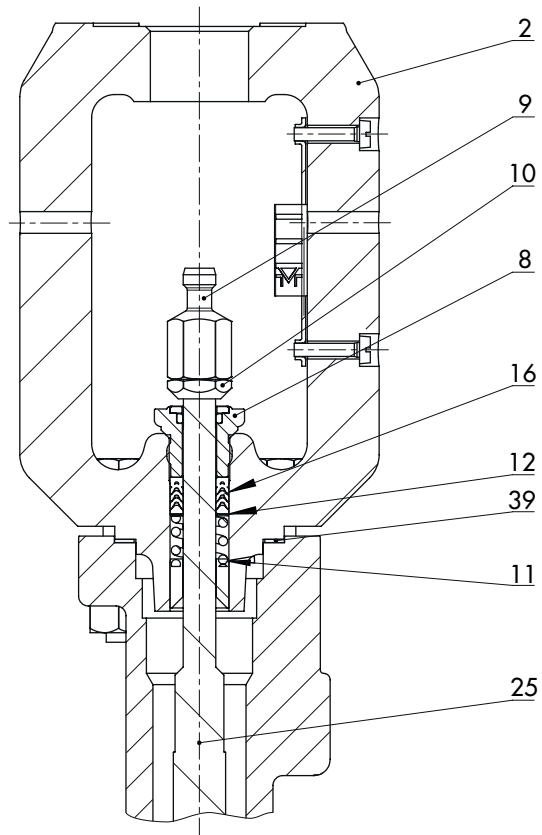
Fig. 3: Intermediate piece
