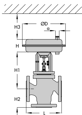
Type 3244 Valve with Type 3271 Actuator
