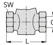
Version with female thread
