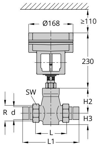
Type 3222/2780-2: DN 15 to 50
