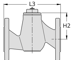
Version with flanged body
