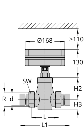
Type 3222/2780-1: DN 15 to 50
