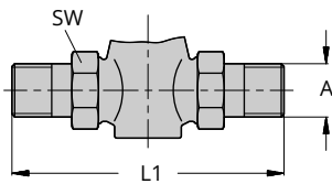
Version with male thread connection and threaded ends
