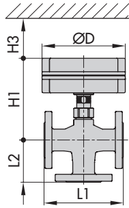
Type 3260/2780-1 DN 15 to 50
