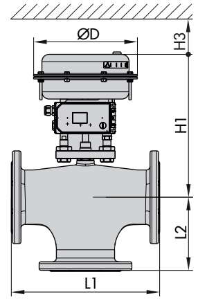
Type 3260/3372 (350 cm²) DN 100 to 150
