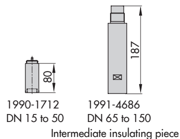
Types 3260/3374-10 and -11 DN 65 to 150
