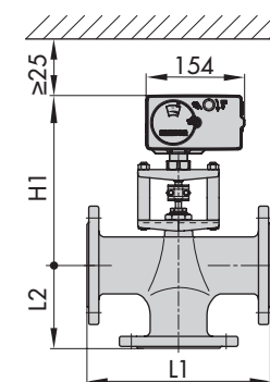
Type 3260/5827-N3 DN 65 and 80
