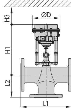
Type 3260/3372 (120 cm²) DN 65 to 80
