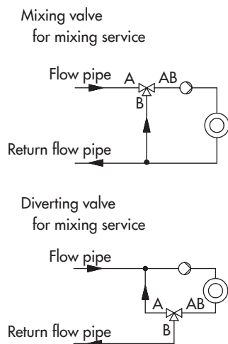
Fig. 5: Functional drawing of Type 3260 as a mixing valve (left) and diverting valve (right)
