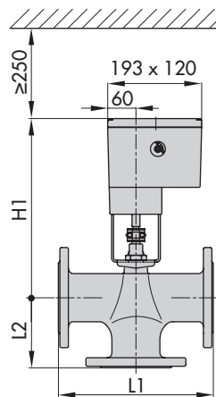
Types 3260/3374-10 and -11 DN 65 to 150
