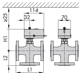
Type 3260/5857, Type 3260/5757-7 DN 15 to 25
