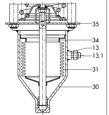
Bellows actuator: 30 to 85 psi · 75 to 145 psi
