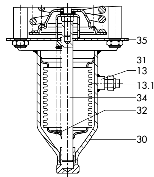
Bellows actuator: 145 to 320 psi · 300 to 400 psi
