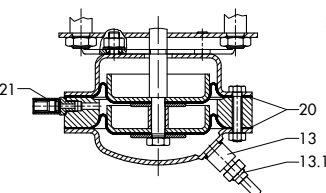
Diaphragm actuator with two diaphragms for increased safety
