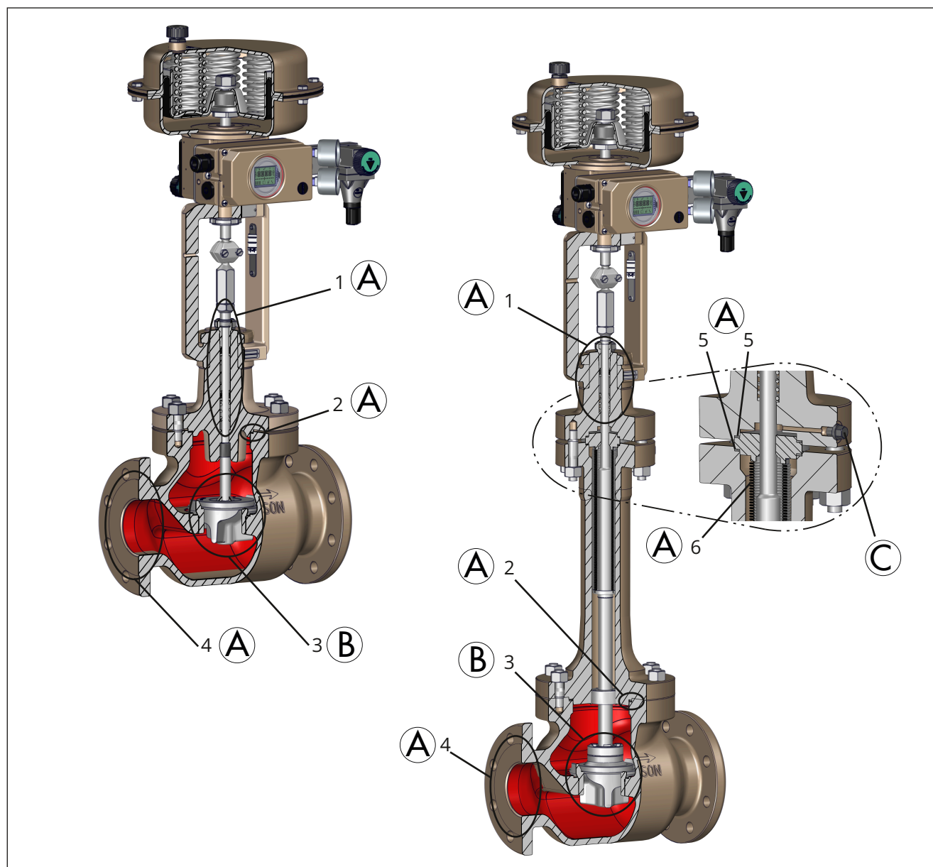
Fig. 27: Possible points of leakage on the control valve: Version with standard bonnet (left) and version with bellows seal (right), which also applies to versions with insulating section or intermediate piece.
