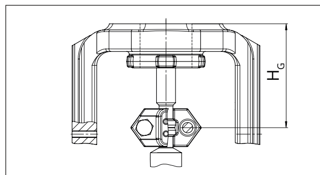
Fig. 25: Stem connector/yoke dimension
