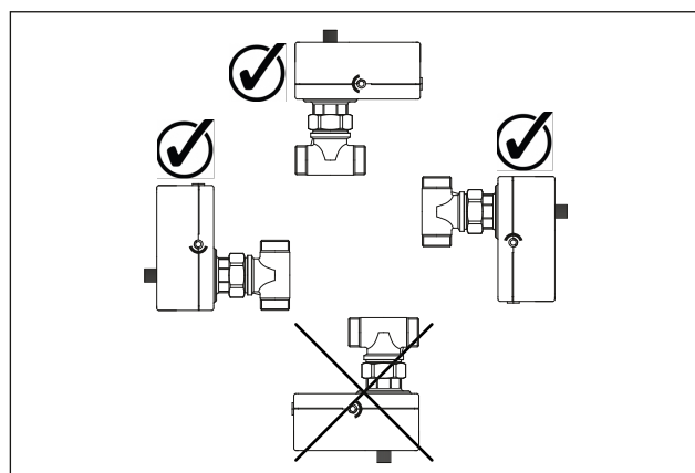
Fig. 4: Mounting position
