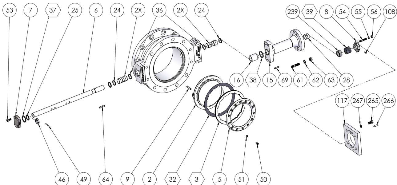
Fig. 10: Exploded drawing of the control and shut-off butterfly valve
