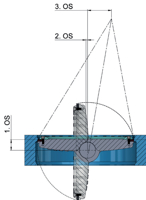
Fig. 3: Triple eccentricity
