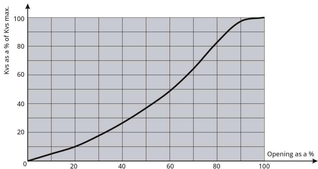
Fig. 5: Kvs-characteristic curve diagram
