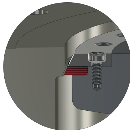
Fig. 4: Seat version
