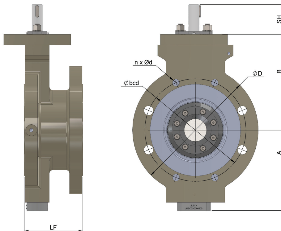
Fig. 8: Butterfly valve with a double-flange design
